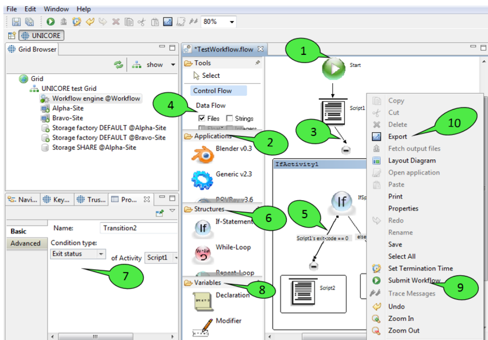
Figure 11: The workflow editor: editing mode
