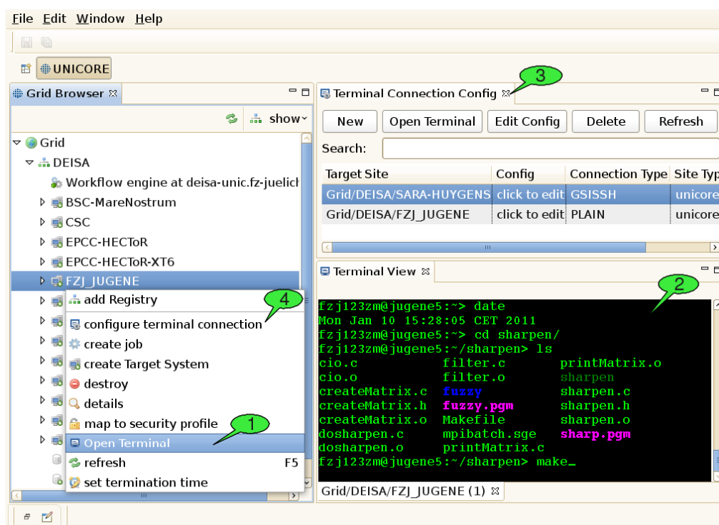
Figure 13: Opening and using terminal connections.
