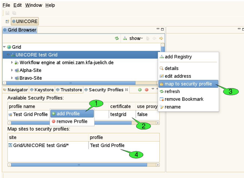
Figure 15: The Security Profiles view
