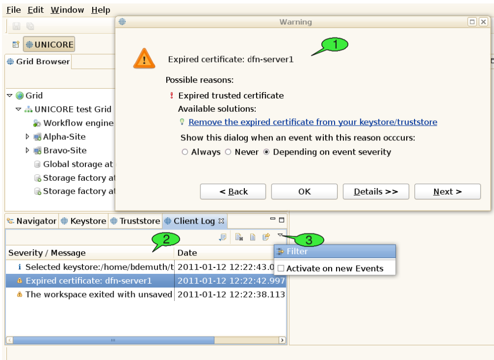
Figure 14: Event dialogs and client log
