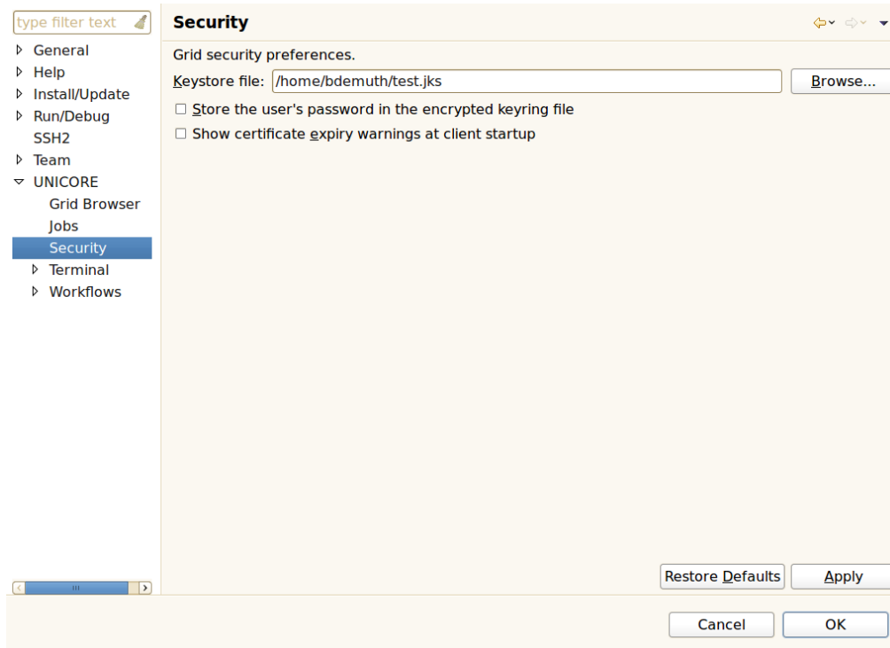
Figure 26: Security related preferences
