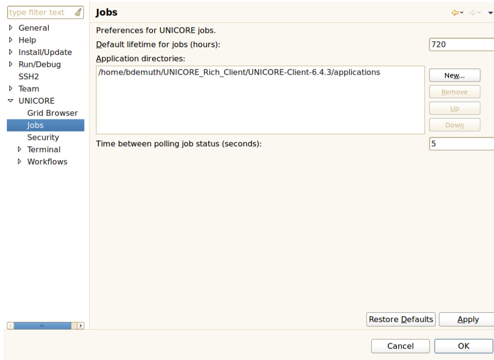
Figure 25: Preferences regarding installed application GUIs and job descriptions
