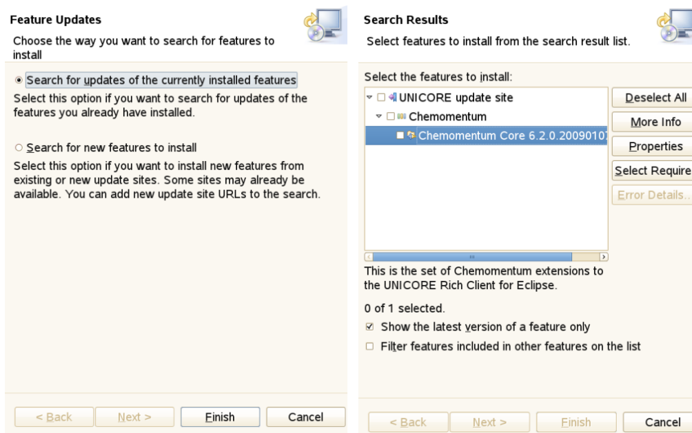
Figure 21: Update the client
