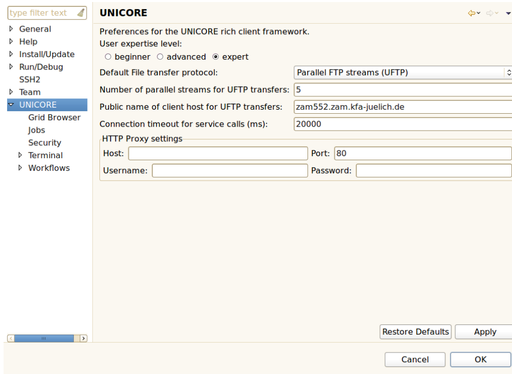
Figure 23: UNICORE related preferences
